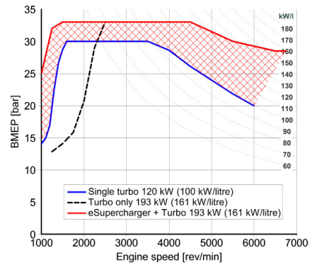
>> Torque curve for MAHLE eSupercharged
